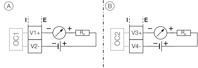
Fig. 35: (I = internal, E = external, R_B = load)
