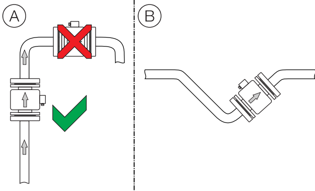
Fig. 19: Free inlet or outlet
