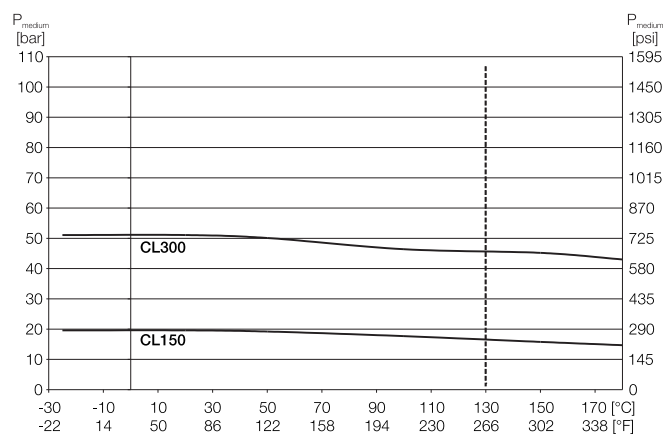
Fig. 9: ASME flange, steel, up to DN 400 (16") (CL150/300); up to DN 1000 (40") (CL150); design level "A"
