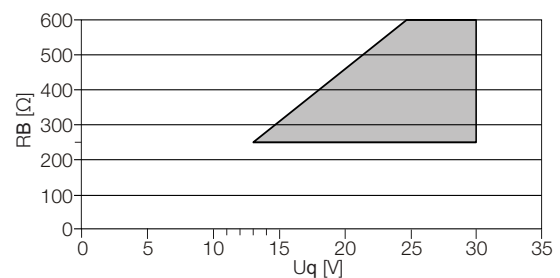
Fig. 33: Source voltage for passive outputs
