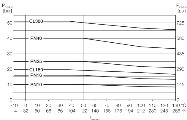
Fig. 15: Welded steel housing, DN 25 ... 600 (1 ... 24"); design level "B"
