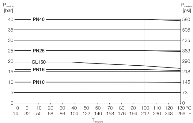
Fig. 14: Cast iron housing, DN 25 ... 600 (1 ... 24"); design level "B"
