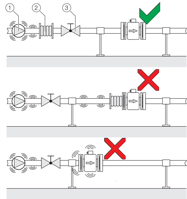
Fig. 21: Vibration damping
