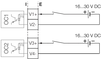
Fig. 38: Plug-in card as digital input (I = internal, E = external)
