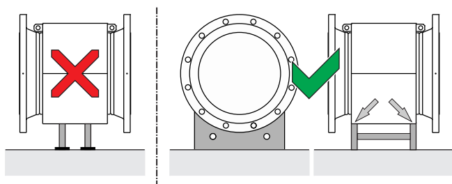
Fig. 1: Support for meter sizes larger than DN 400
