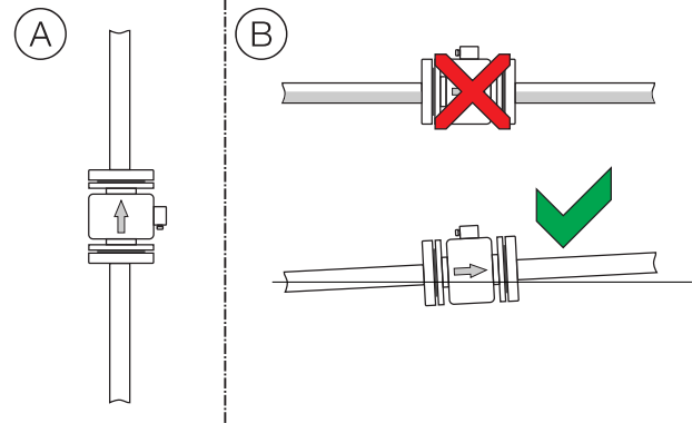
Fig. 17: Mounting position
