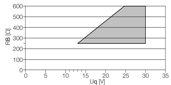
Fig. 36: Source voltage for passive outputs
