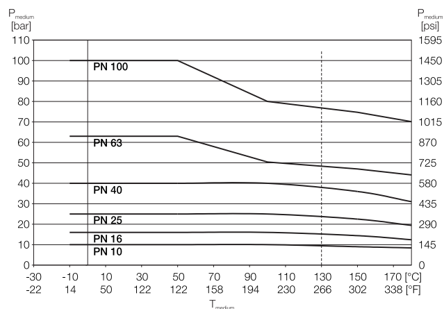
Fig. 8: DIN flange, steel, up to DN 600 (24"); design level "A"
