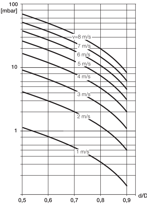
Fig. 5: Flow rate nomogram for pressure drop calculations for flange transition piece with \alpha/2 = 8^\circ
