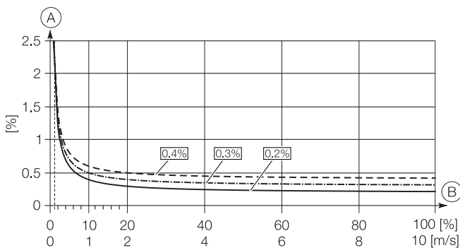
Fig. 5: Measuring error
